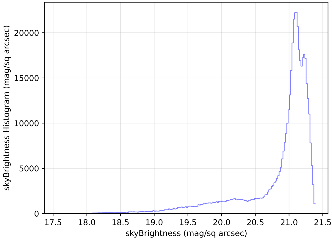
noroll_mjdp60_v3.4_10yrs All sky r band: skyBrightness Histogram
