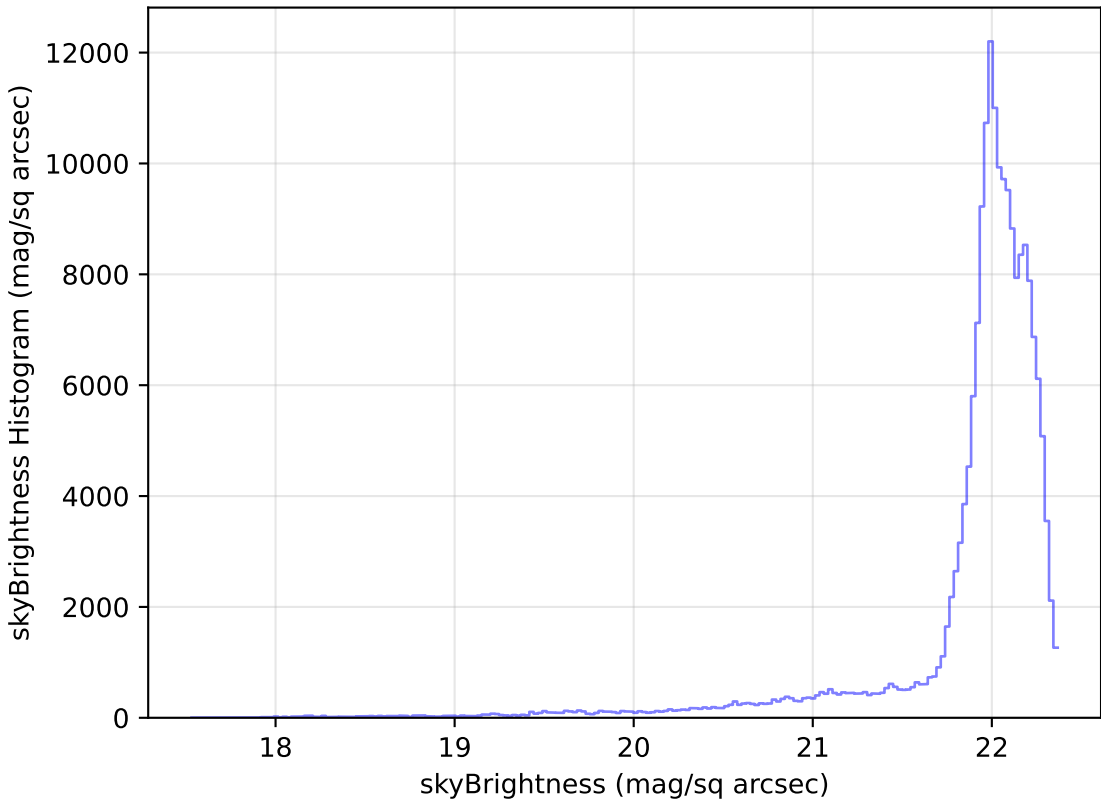
noroll_mjdp60_v3.4_10yrs All sky g band: skyBrightness Histogram
