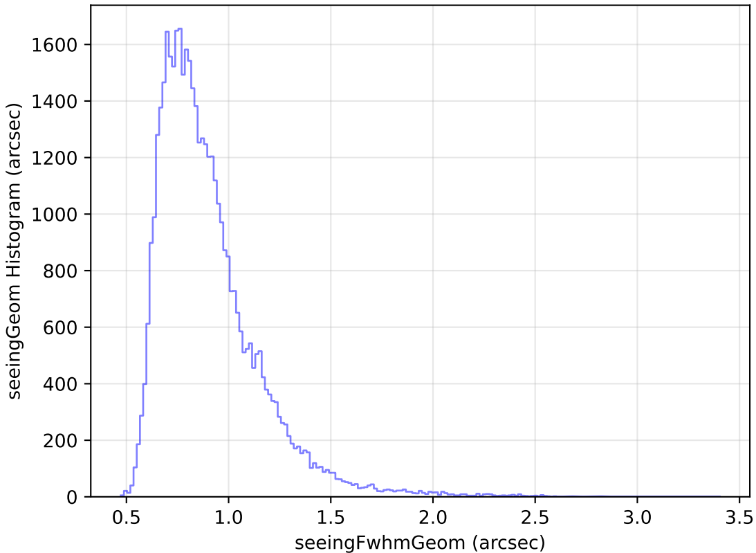
noroll_mjdp60_v3.4_10yrs Yr 1 z band: seeingGeom Histogram
