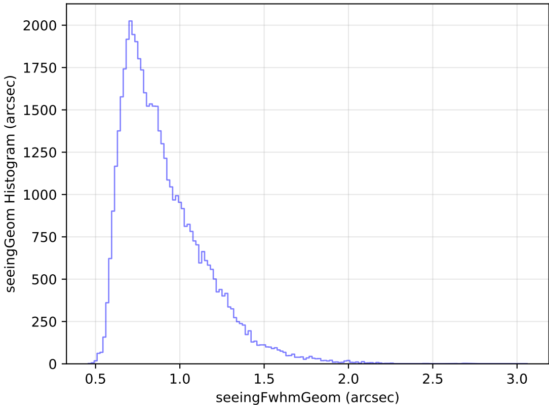
noroll_mjdp60_v3.4_10yrs Yr 1 r band: seeingGeom Histogram
