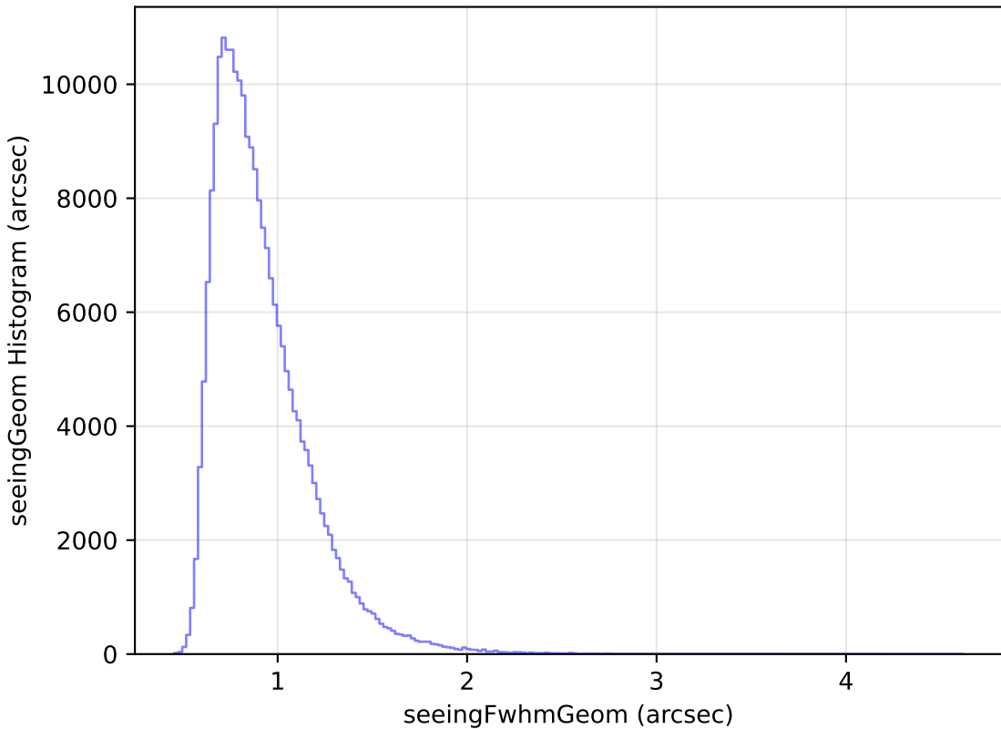
noroll_mjdp60_v3.4_10yrs Yr 1 all bands: seeingGeom Histogram
