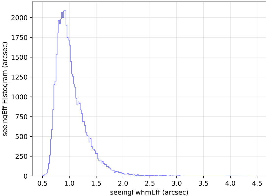
noroll_mjdp60_v3.4_10yrs Yr 1 y band: seeingEff Histogram
