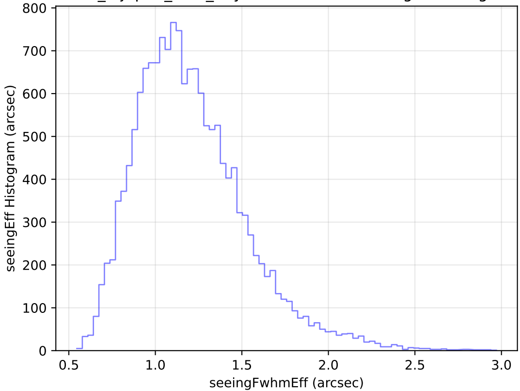
noroll_mjdp60_v3.4_10yrs Yr 1 u band: seeingEff Histogram
