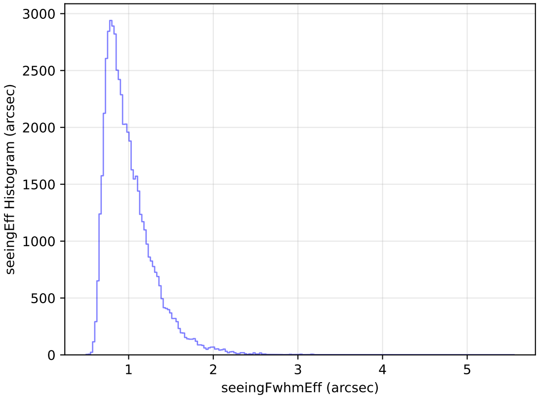
noroll_mjdp60_v3.4_10yrs Yr 1 i band: seeingEff Histogram
