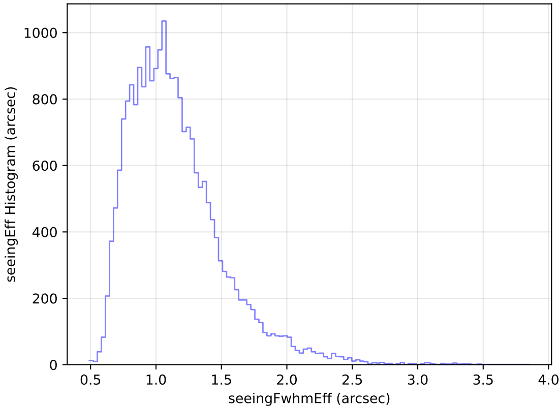
noroll_mjdp60_v3.4_10yrs Yr 1 g band: seeingEff Histogram
