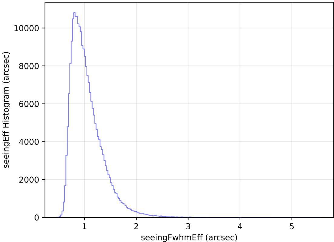
noroll_mjdp60_v3.4_10yrs Yr 1 all bands: seeingEff Histogram
