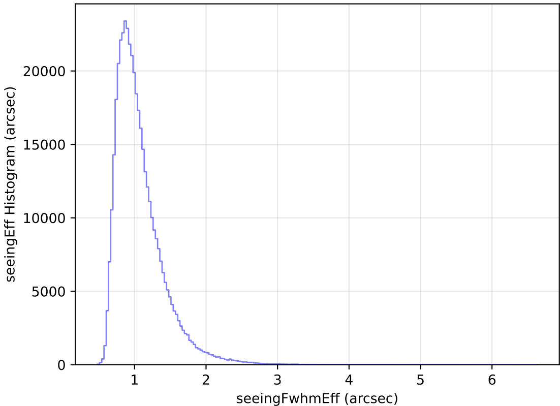
noroll_mjdp60_v3.4_10yrs WFD z band: seeingEff Histogram
