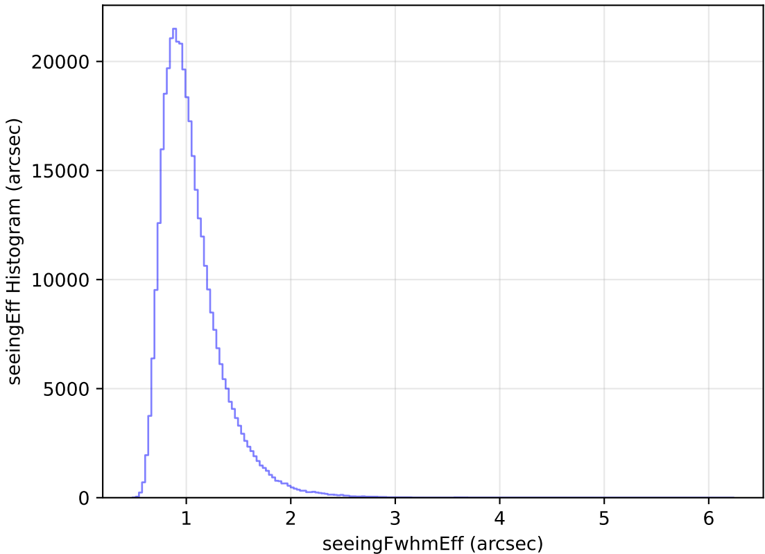
noroll_mjdp60_v3.4_10yrs WFD y band: seeingEff Histogram
