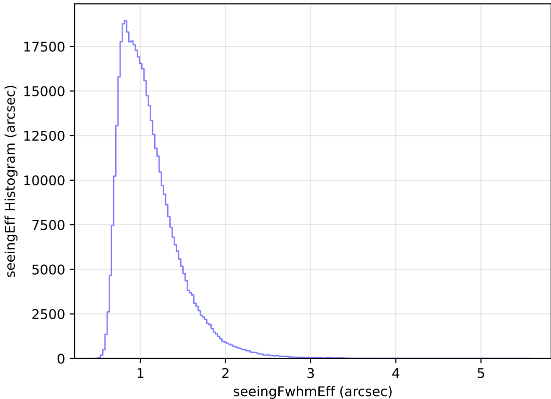
noroll_mjdp60_v3.4_10yrs WFD r band: seeingEff Histogram
