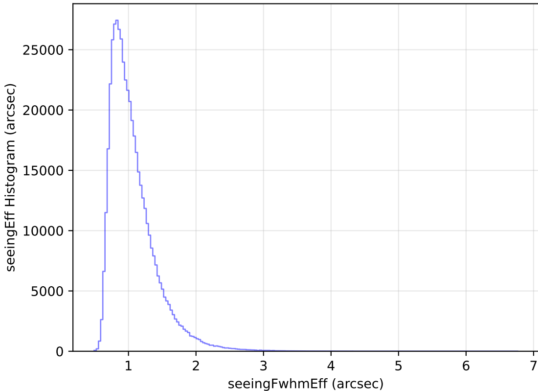
noroll_mjdp60_v3.4_10yrs WFD i band: seeingEff Histogram
