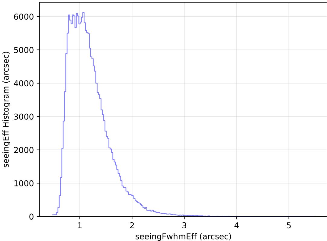
noroll_mjdp60_v3.4_10yrs WFD g band: seeingEff Histogram
