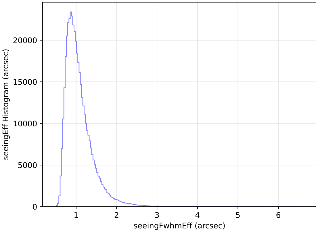
noroll_mjdp60_v3.4_10yrs All sky z band: seeingEff Histogram
