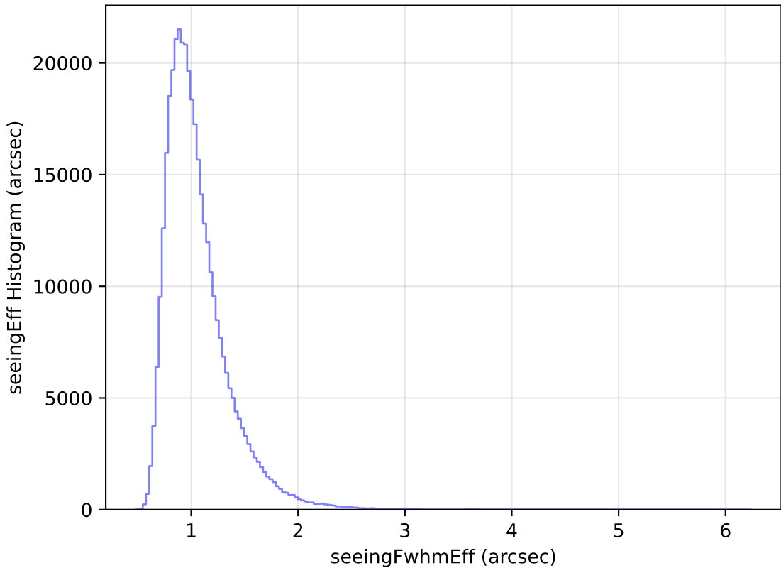
noroll_mjdp60_v3.4_10yrs All sky y band: seeingEff Histogram
