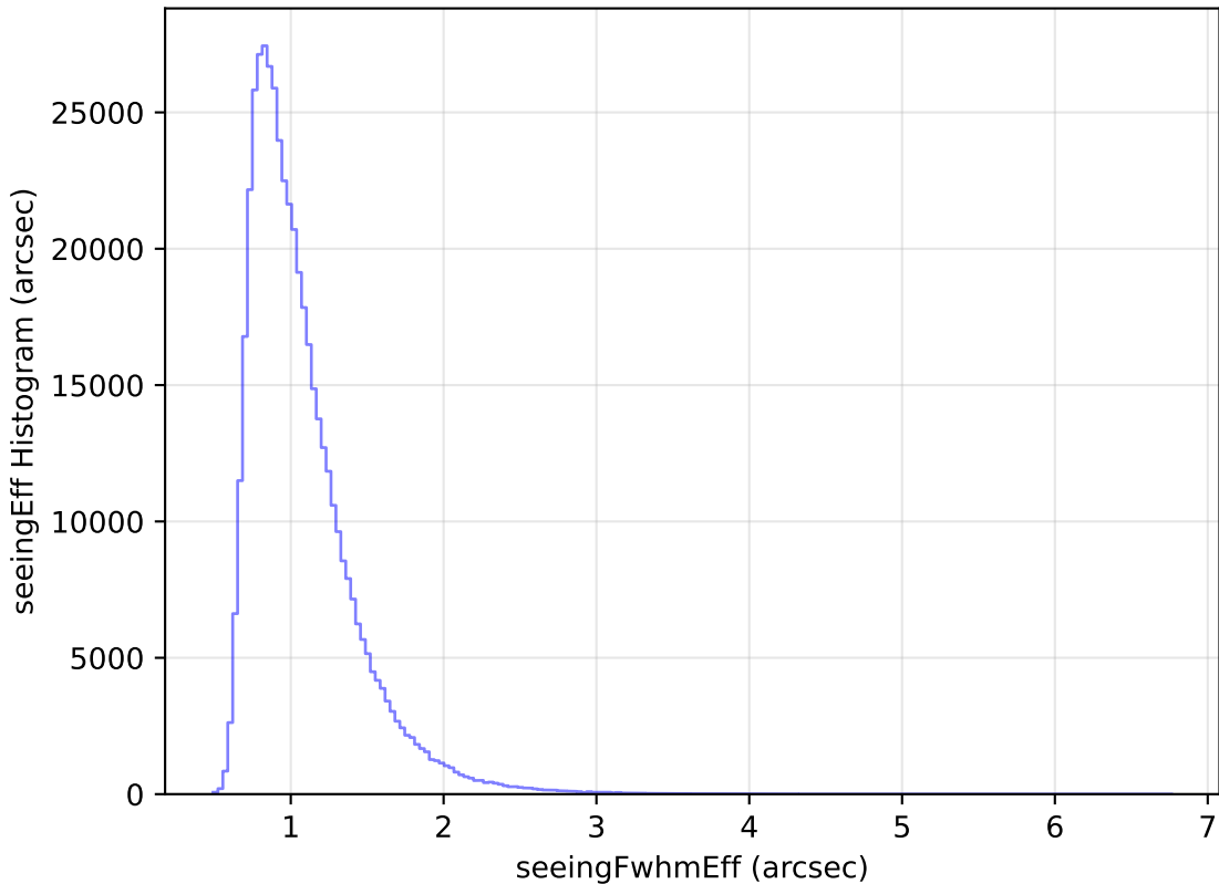
noroll_mjdp60_v3.4_10yrs All sky i band: seeingEff Histogram
