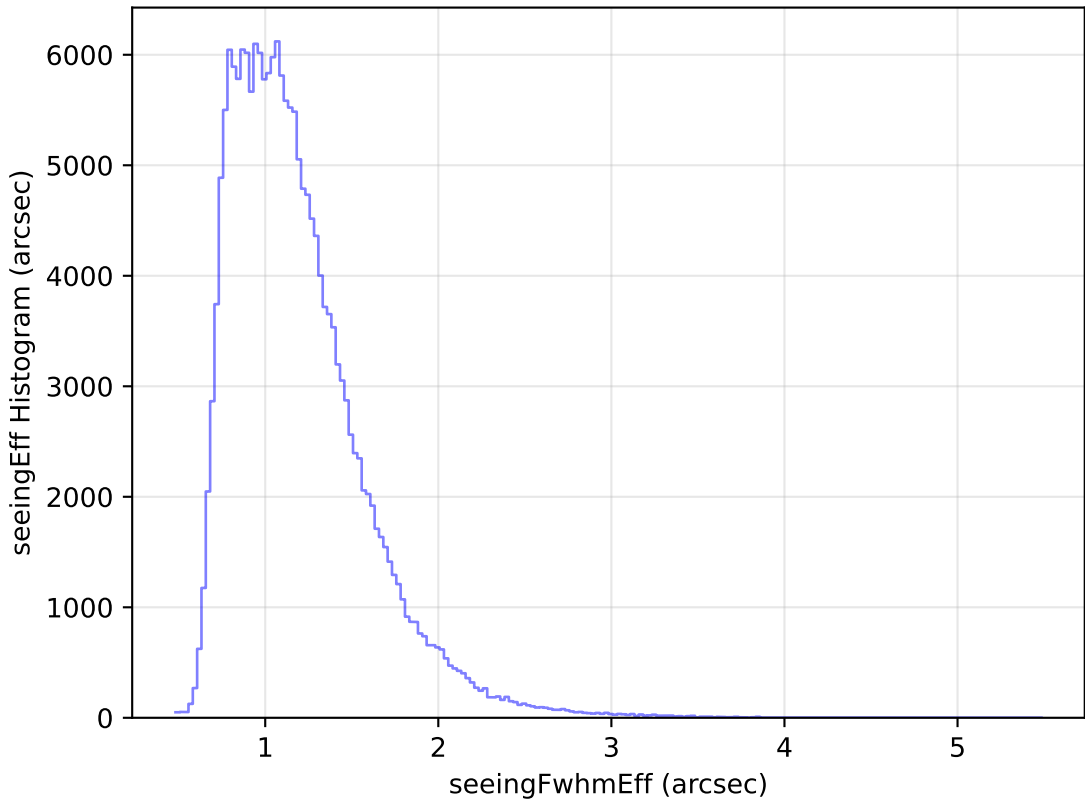
noroll_mjdp60_v3.4_10yrs All sky g band: seeingEff Histogram
