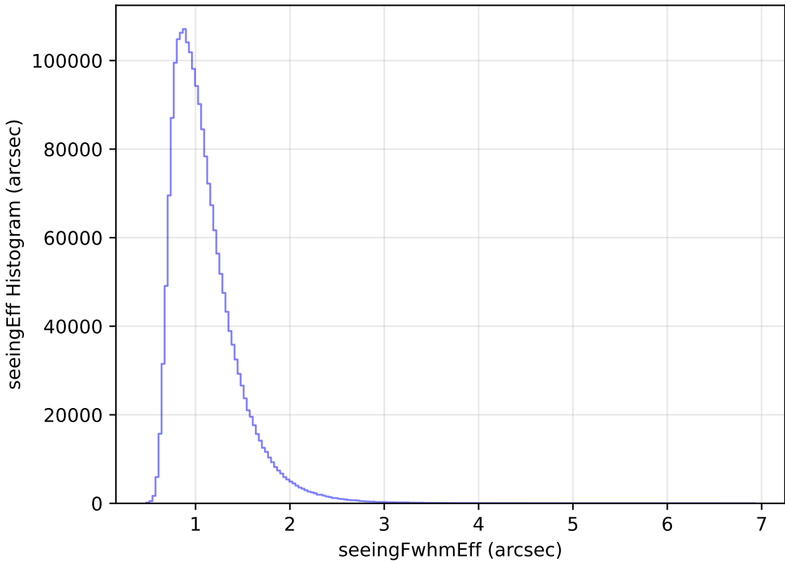
noroll_mjdp60_v3.4_10yrs All sky all bands: seeingEff Histogram
