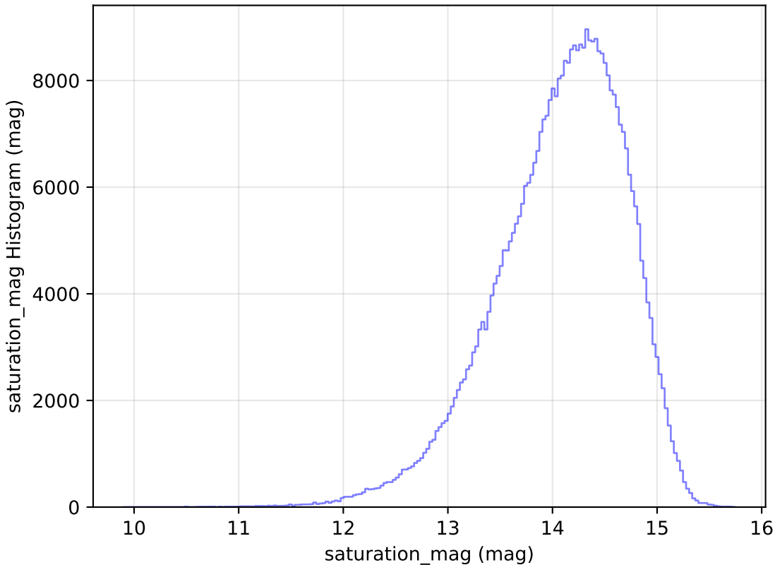
noroll_mjdp60_v3.4_10yrs WFD z band: saturation_mag Histogram
