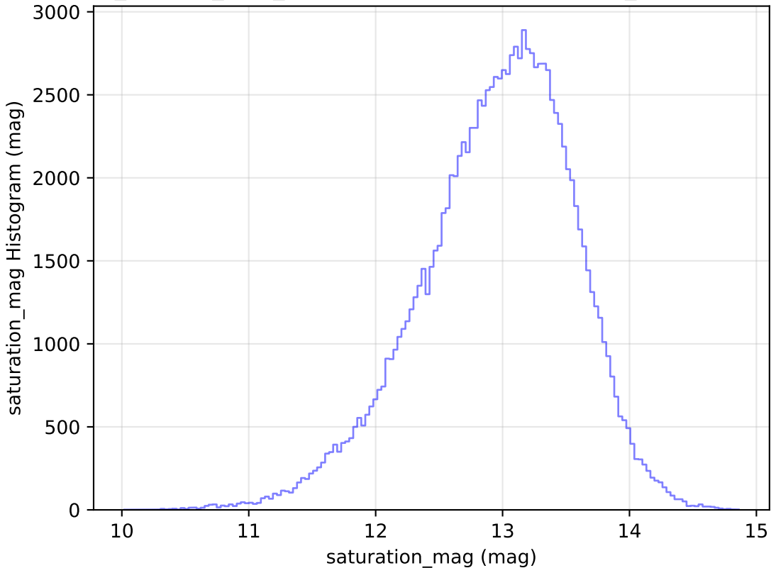
noroll_mjdp60_v3.4_10yrs WFD u band: saturation_mag Histogram
