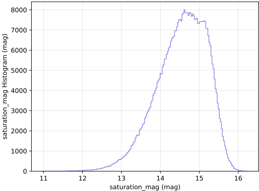
noroll_mjdp60_v3.4_10yrs WFD r band: saturation_mag Histogram
