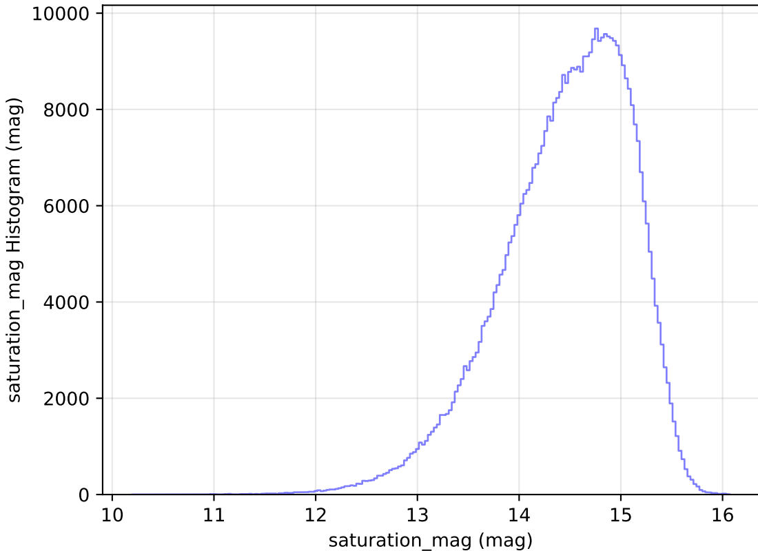
noroll_mjdp60_v3.4_10yrs WFD i band: saturation_mag Histogram
