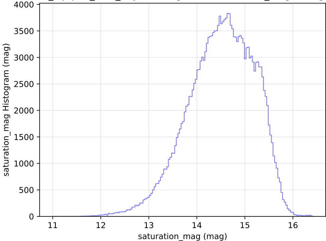
noroll_mjdp60_v3.4_10yrs WFD g band: saturation_mag Histogram
