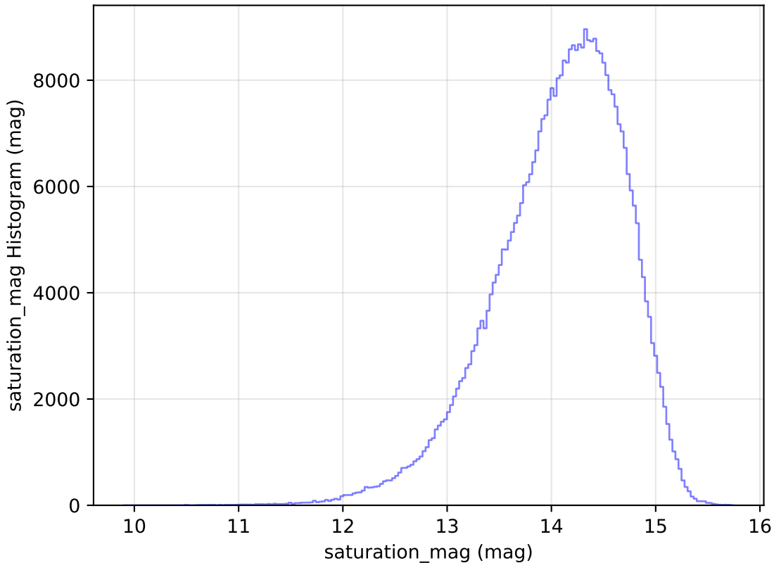
noroll_mjdp60_v3.4_10yrs All sky z band: saturation_mag Histogram
