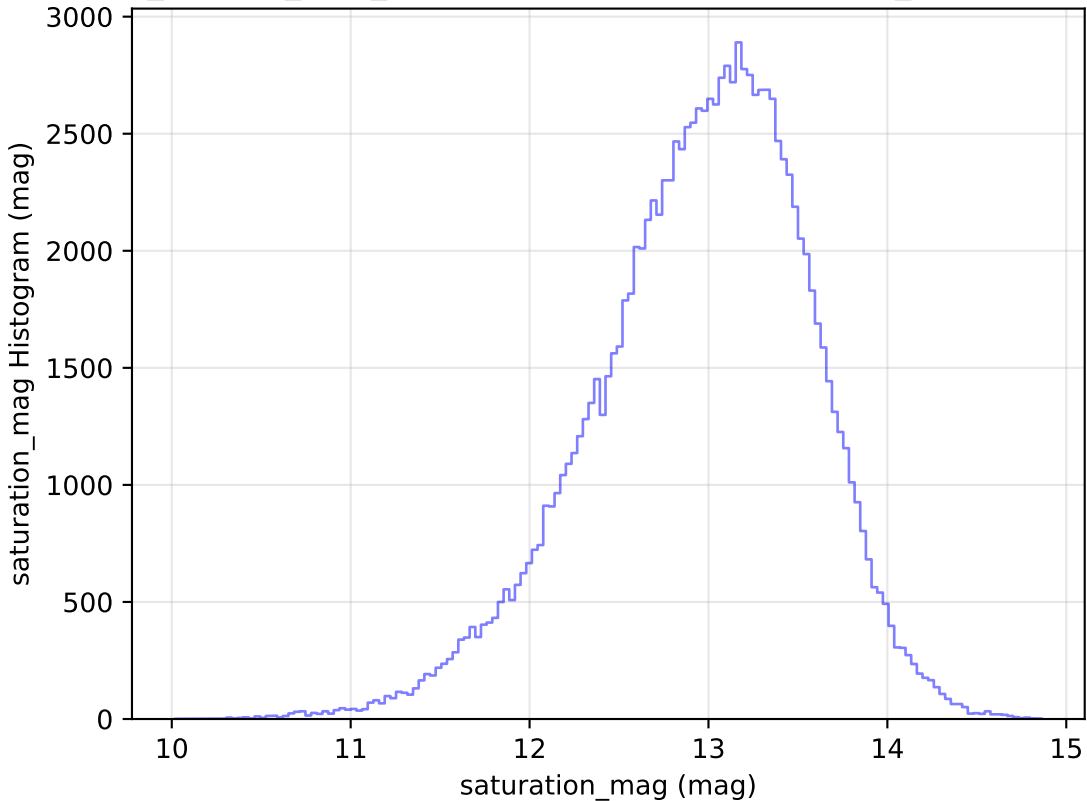
noroll_mjdp60_v3.4_10yrs All sky u band: saturation_mag Histogram
