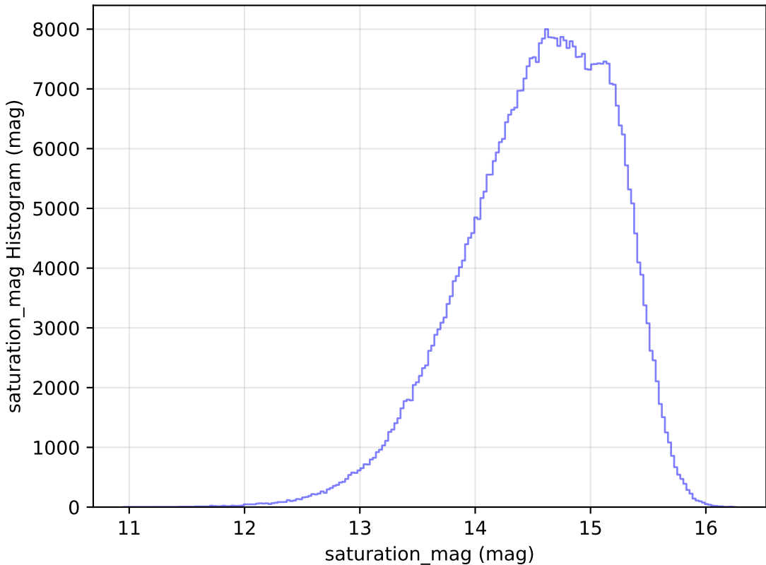
noroll_mjdp60_v3.4_10yrs All sky r band: saturation_mag Histogram
