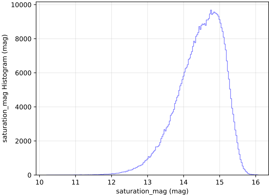
noroll_mjdp60_v3.4_10yrs All sky i band: saturation_mag Histogram
