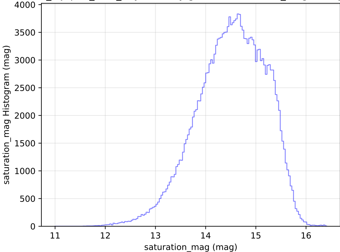
noroll_mjdp60_v3.4_10yrs All sky g band: saturation_mag Histogram
