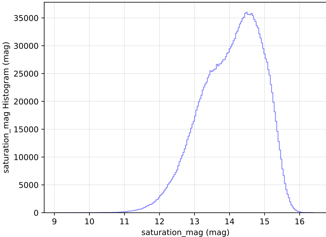
noroll_mjdp60_v3.4_10yrs All sky all bands: saturation_mag Histogram
