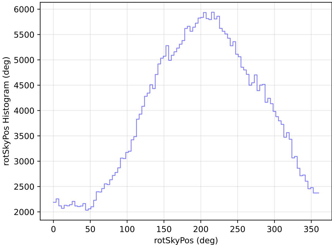
noroll_mjdp60_v3.4_10yrs WFD y band: rotSkyPos Histogram
