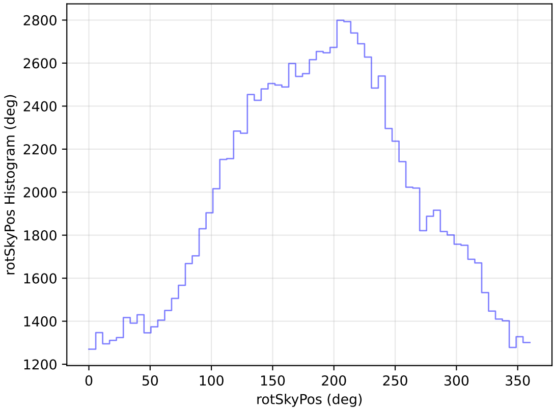
noroll_mjdp60_v3.4_10yrs WFD u band: rotSkyPos Histogram
