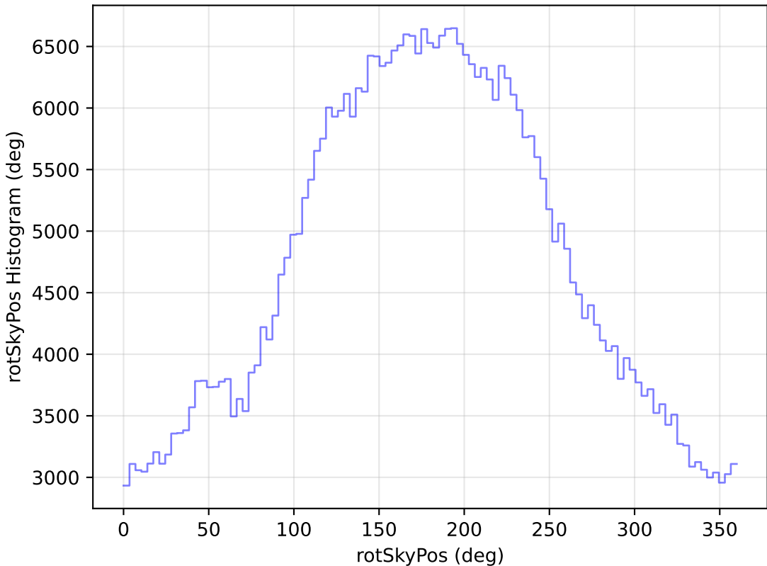
noroll_mjdp60_v3.4_10yrs WFD r band: rotSkyPos Histogram
