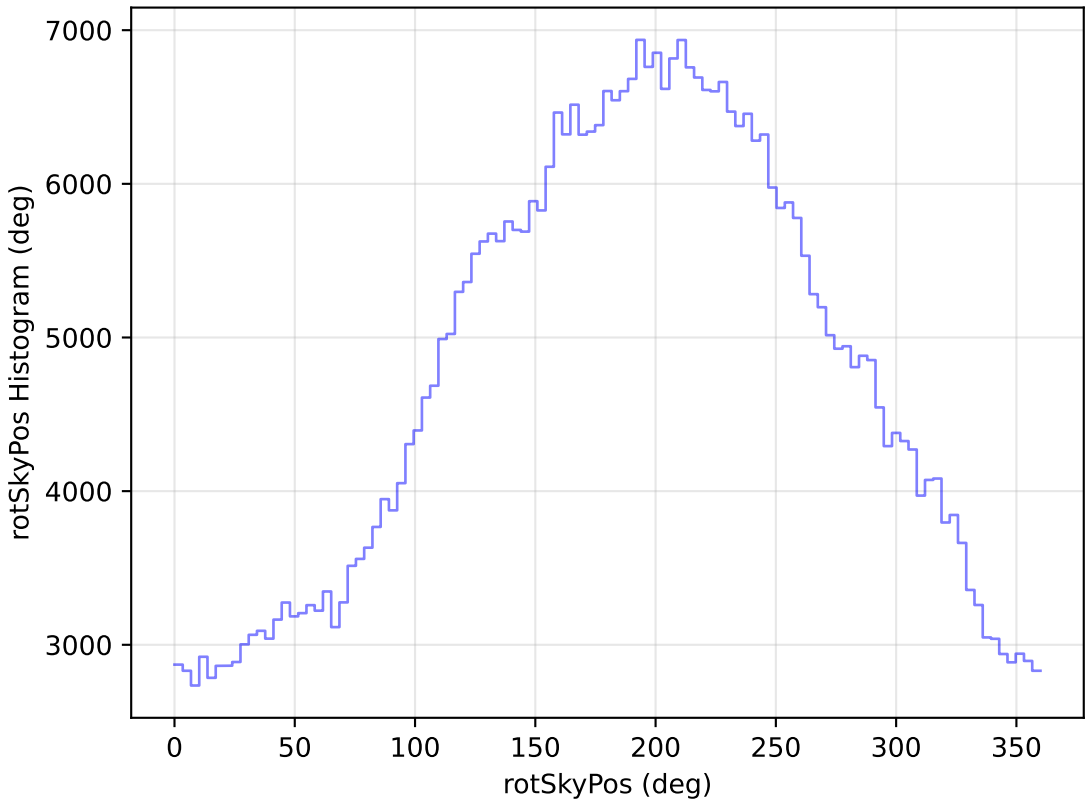
noroll_mjdp60_v3.4_10yrs WFD i band: rotSkyPos Histogram
