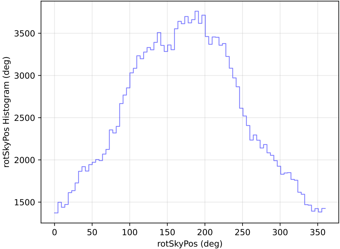
noroll_mjdp60_v3.4_10yrs WFD g band: rotSkyPos Histogram
