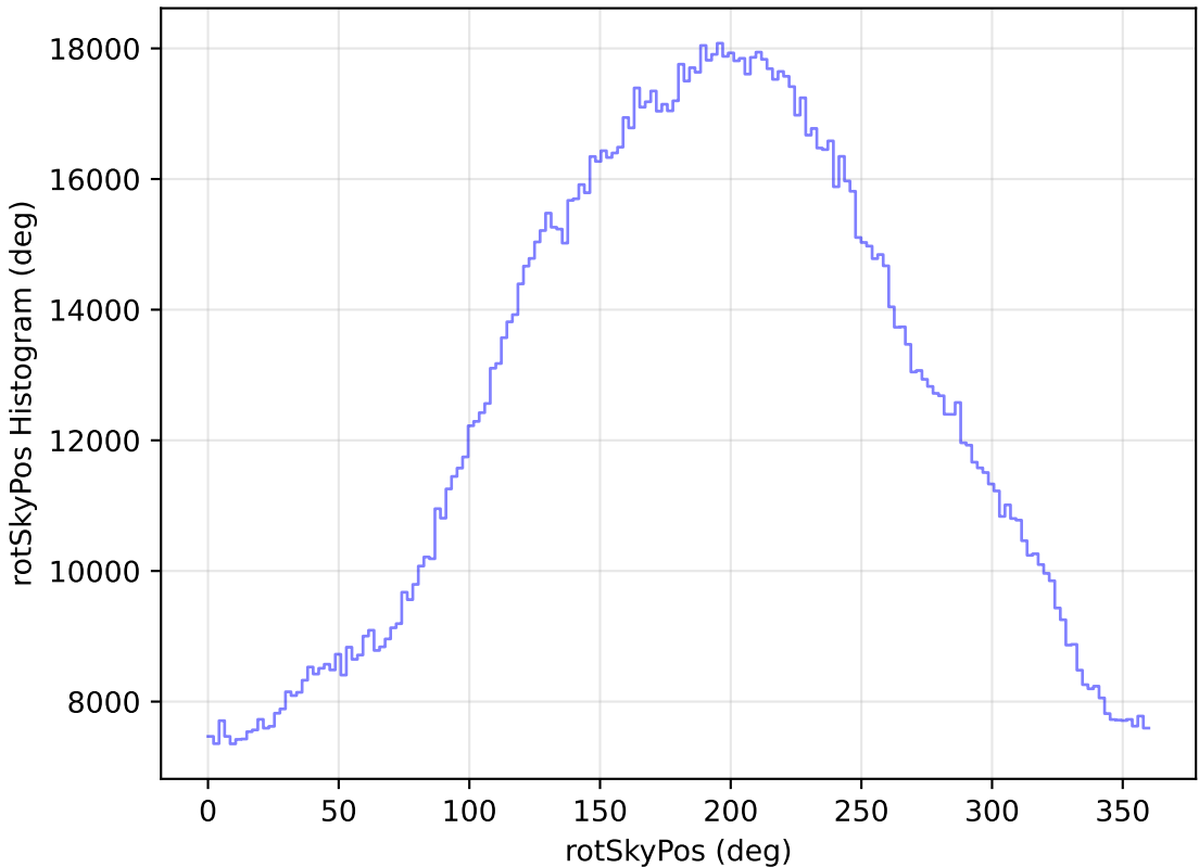
noroll_mjdp60_v3.4_10yrs WFD all bands: rotSkyPos Histogram
