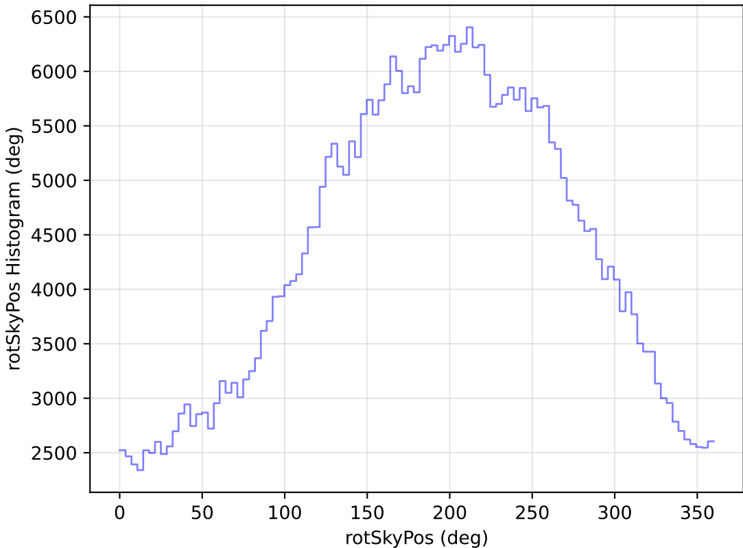
noroll_mjdp60_v3.4_10yrs All sky z band: rotSkyPos Histogram
