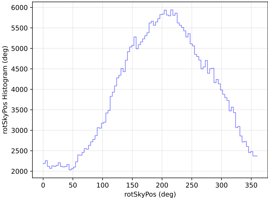
noroll_mjdp60_v3.4_10yrs All sky y band: rotSkyPos Histogram
