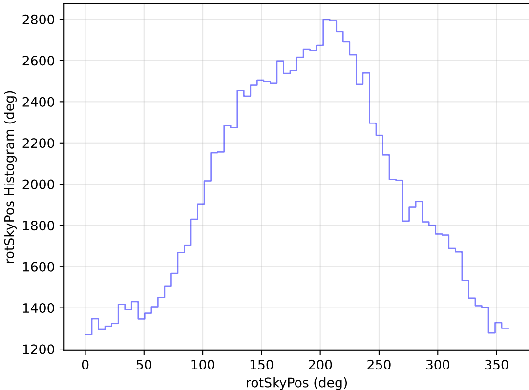
noroll_mjdp60_v3.4_10yrs All sky u band: rotSkyPos Histogram
