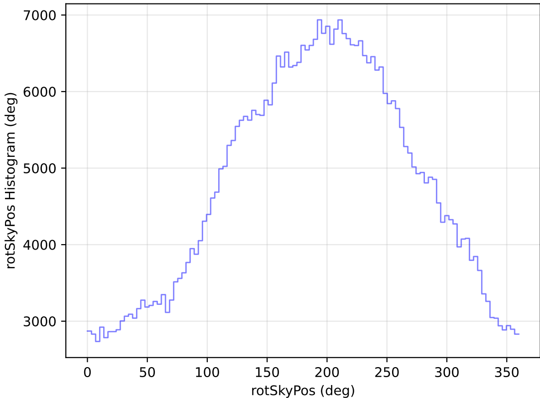
noroll_mjdp60_v3.4_10yrs All sky i band: rotSkyPos Histogram
