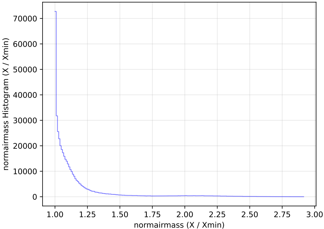
noroll_mjdp60_v3.4_10yrs WFD z band: normairmass Histogram
