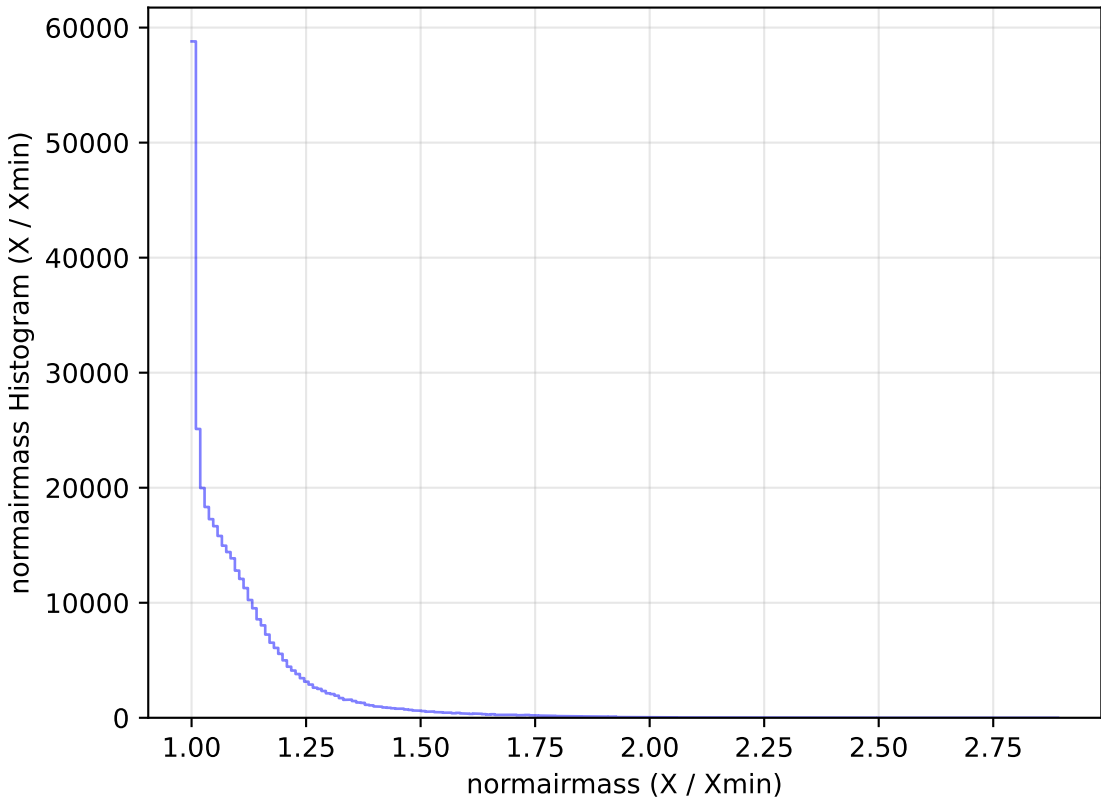
noroll_mjdp60_v3.4_10yrs WFD y band: normairmass Histogram
