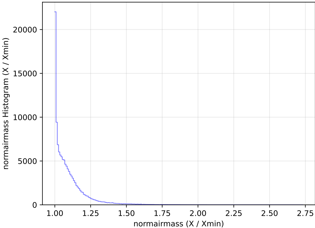
noroll_mjdp60_v3.4_10yrs WFD u band: normairmass Histogram
