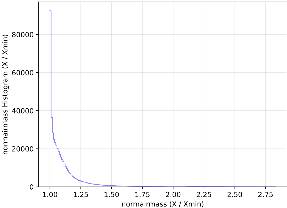
noroll_mjdp60_v3.4_10yrs WFD r band: normairmass Histogram
