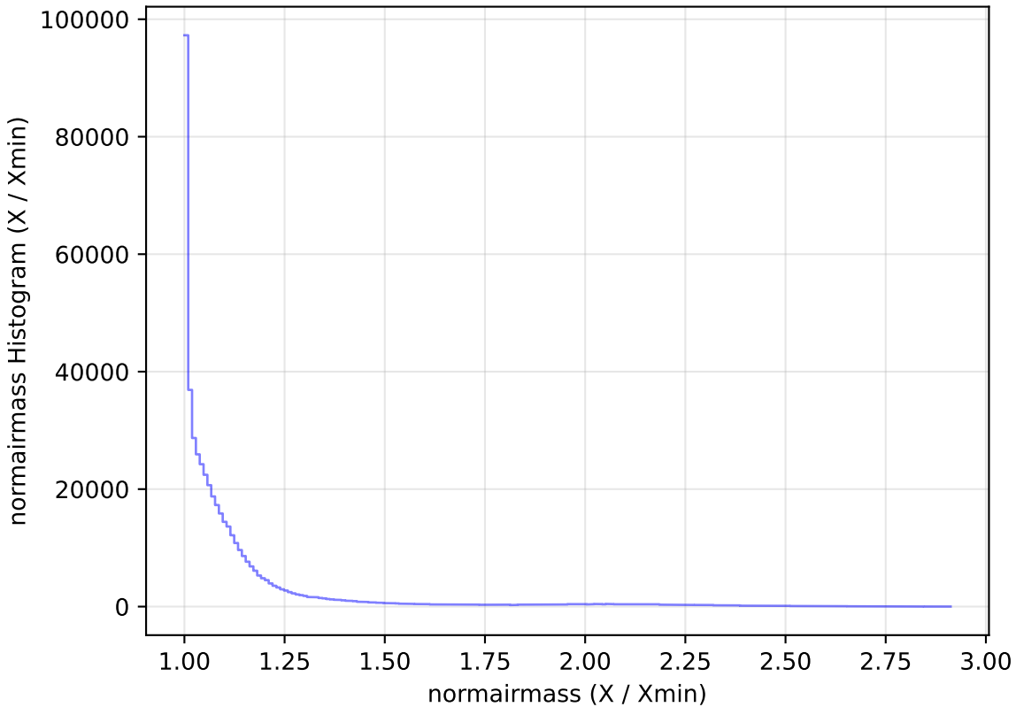
noroll_mjdp60_v3.4_10yrs WFD i band: normairmass Histogram
