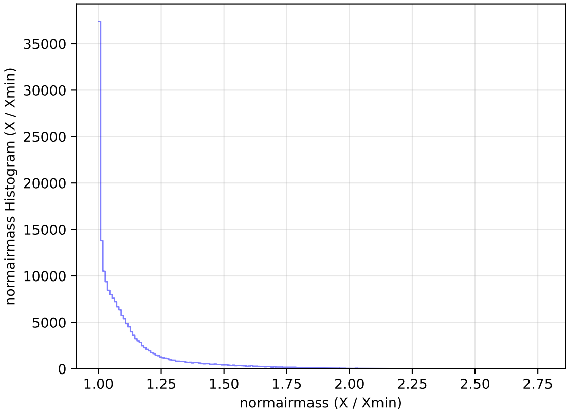
noroll_mjdp60_v3.4_10yrs WFD g band: normairmass Histogram
