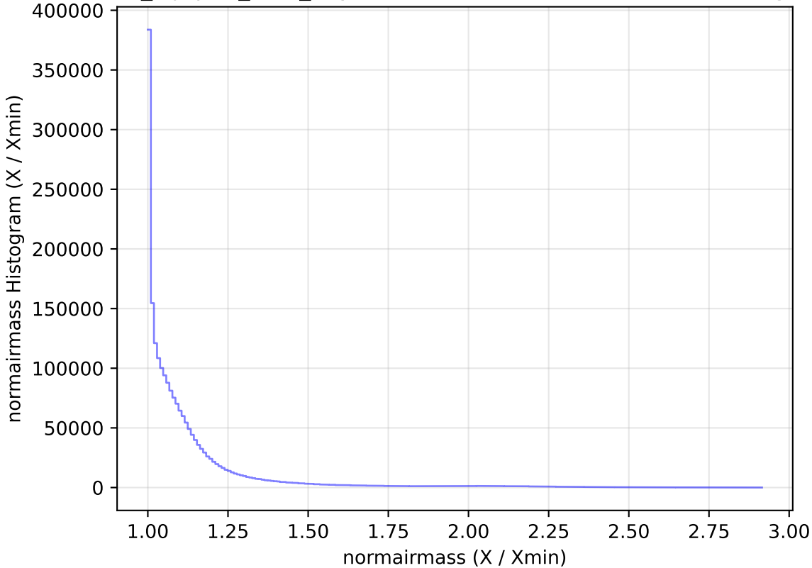
noroll_mjdp60_v3.4_10yrs WFD all bands: normairmass Histogram
