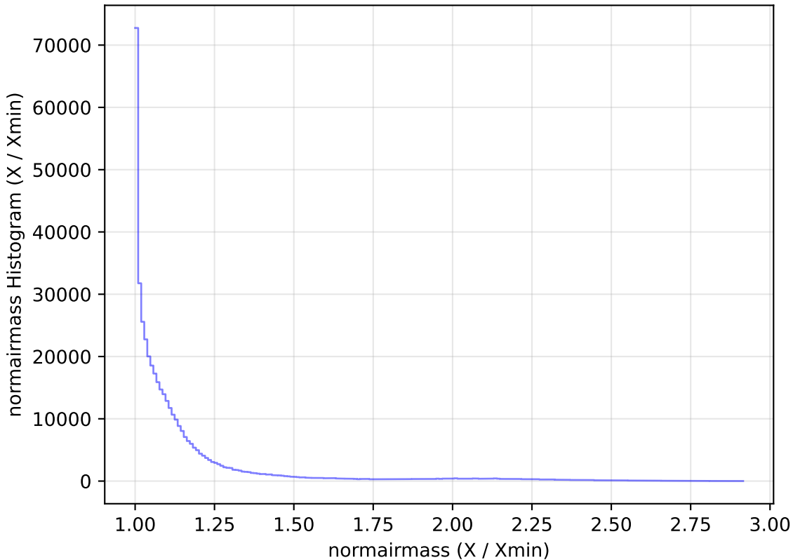
noroll_mjdp60_v3.4_10yrs All sky z band: normairmass Histogram
