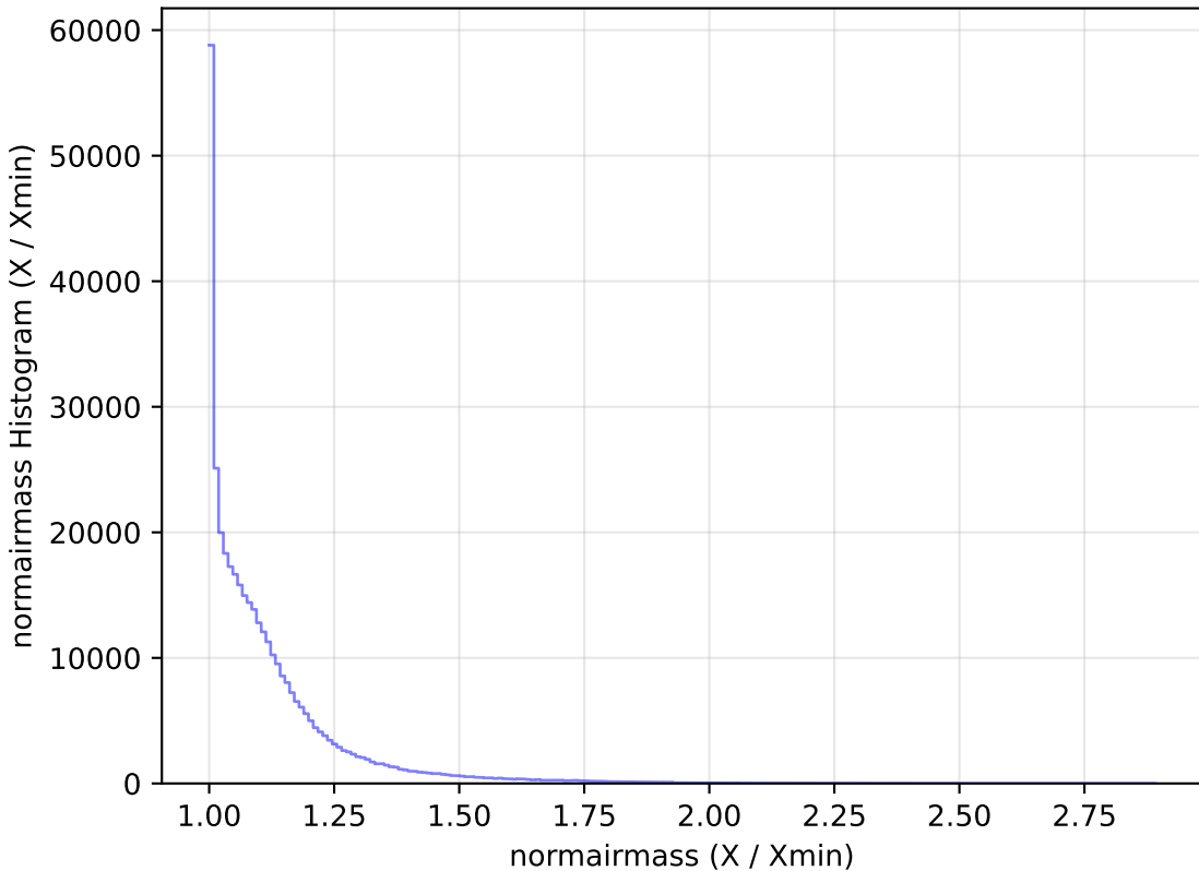
noroll_mjdp60_v3.4_10yrs All sky y band: normairmass Histogram
